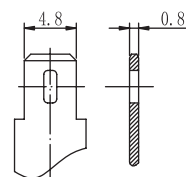
Terminal T1
